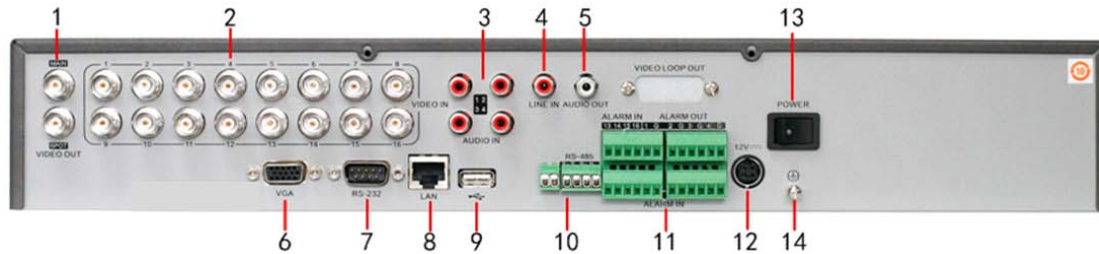
Figure 12. VC-SYS-16H301A Rear Panel
