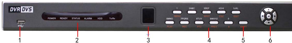
Figure 6. VC-SYS-8H201A Front Panel
